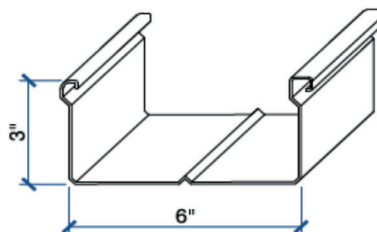
3 x 6 x 0.078 Self Mating Canopy Roof Pan (V-Deck)
